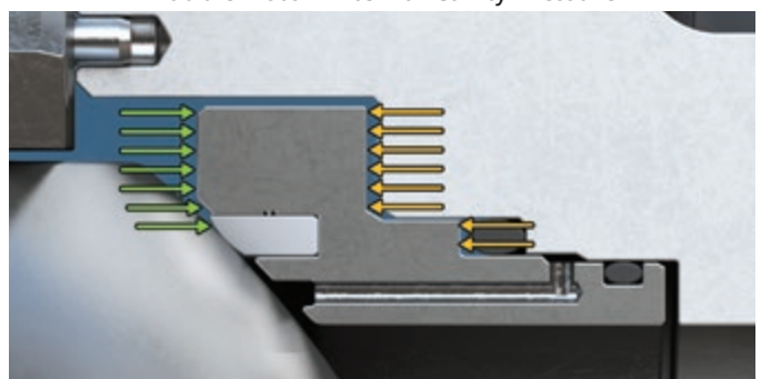
Double Piston Internal Cavity Pressure
